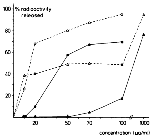
FIG. 3. Leakage of radioactivity contained in TCA-soluble (---) and TCA-insoluble (—) fractions of [ ^3\text{H} ]uridine-labeled HeLa S-3 cells after exposure to various concentrations of AF/013 ( \circ , \bullet ) and the nonionic detergent Triton X-100 ( \Delta , \blacktriangle )
